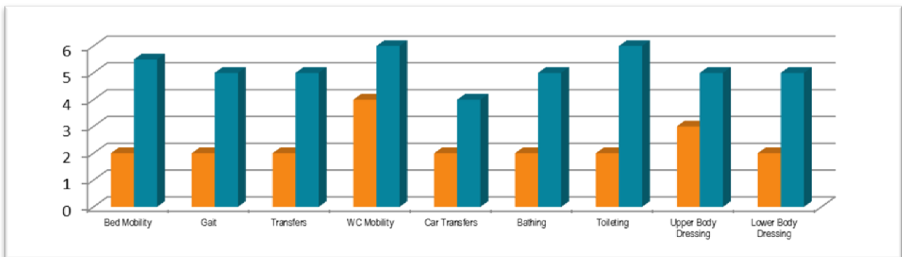
Functional Scores
